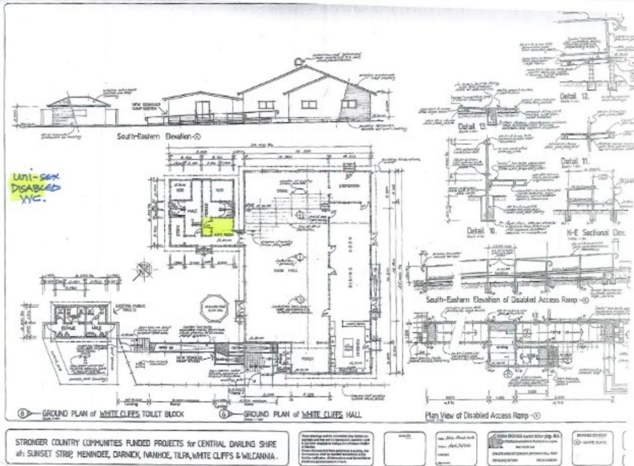
Floor plan and elevations of proposed works for a uni sex disabled toilet amenity in the existing White Cliffs amenity hall.
