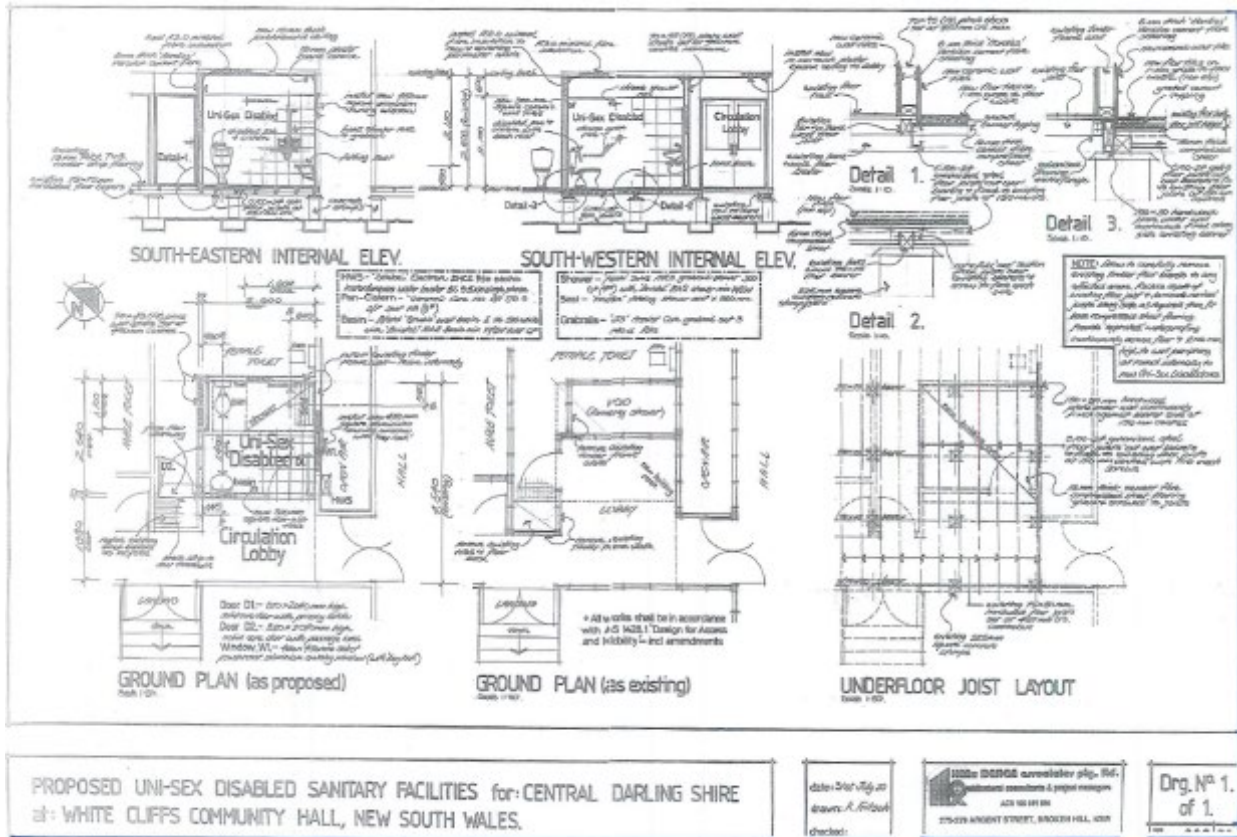
Details of works to uni sex disabled toilets in the existing White Cliffs Community hall.
