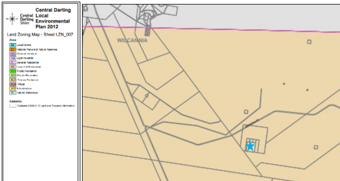
Extract from Central Darling Local Environmental Plan map 007 site Lot 1 in DP 756998
