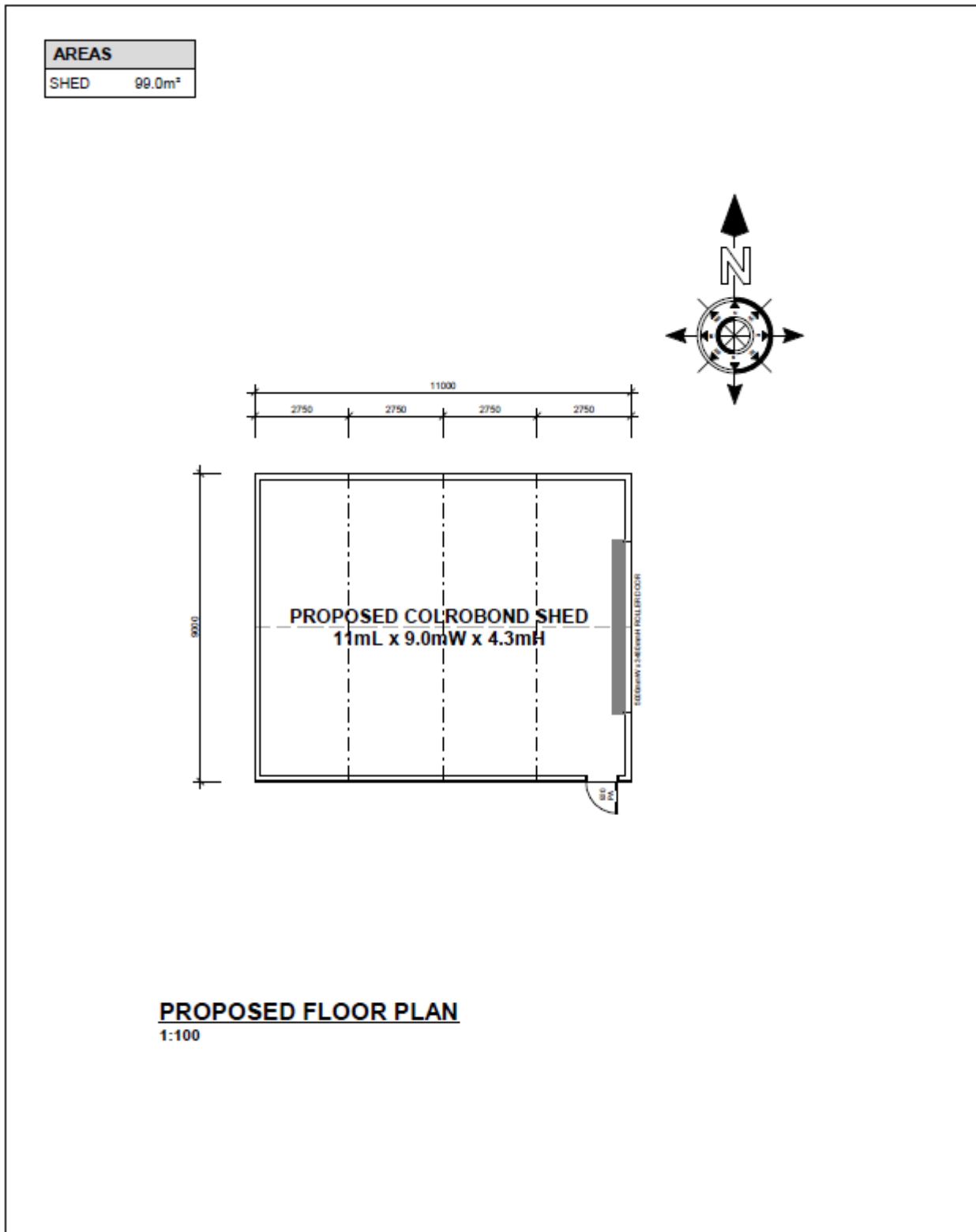
Site plan of the 3 Woore Street/ McIntyre Street Wilcannia NSW 2836 (source Golsworthy Consultants SEE 2021)
