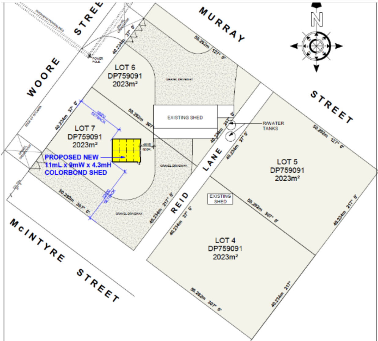
Site plan for the proposed new shed at the National parks depot.- 3 Woore Street/ McIntyre Street Wilcannia NSW 2836 (source Golsworthy Consultants SEE 2021)
